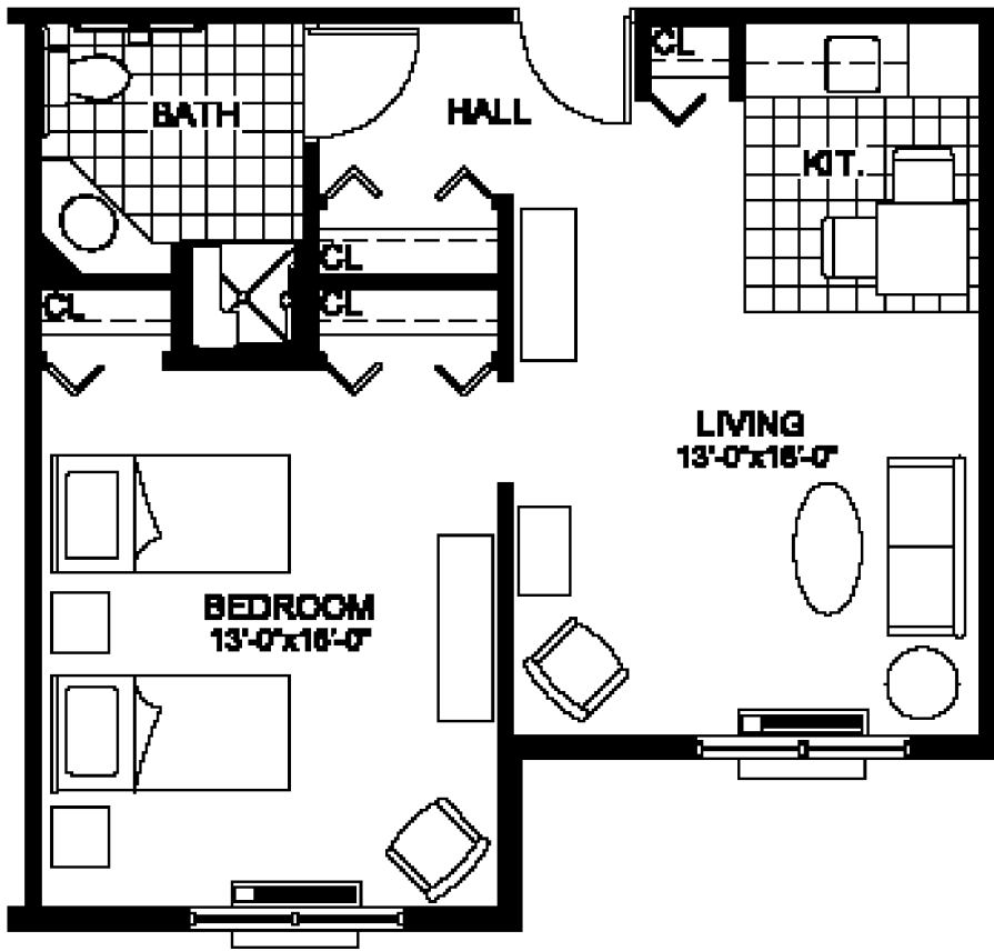
THE BREIDENHART I 630 sq. ft. first floor
