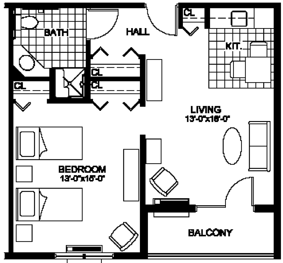
THE BREIDENHART II 630 sq. ft. second floor
